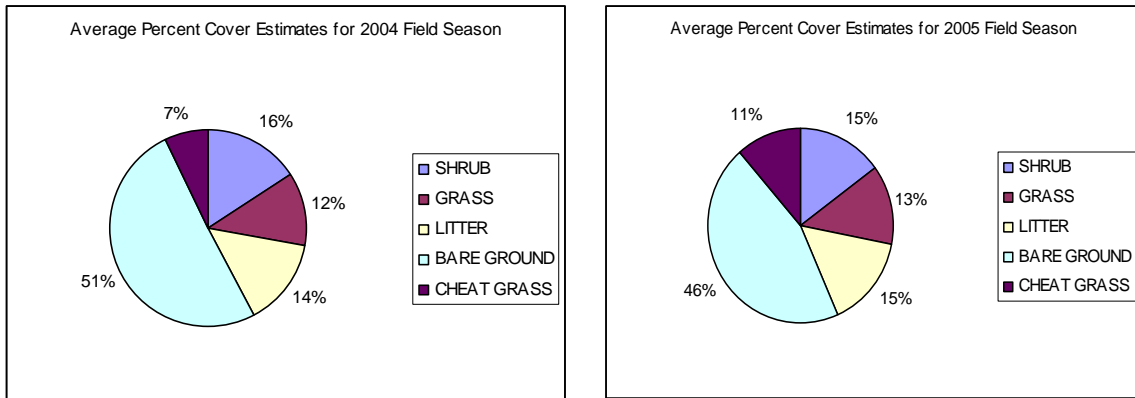
Figure 3: Variations from 2004 to 2005 in the mean percent cover of the five cover types observed in the field
