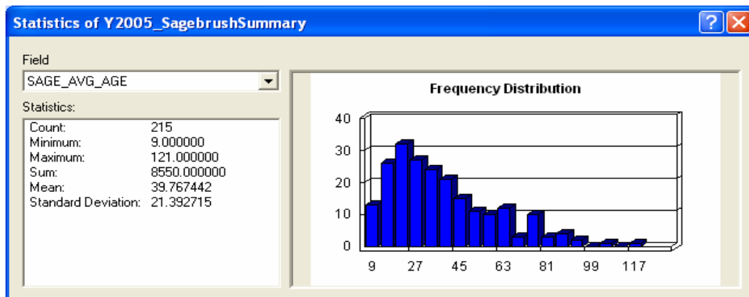
Figure 2: Age distribution of Big Sagebrush in the study area 2005
